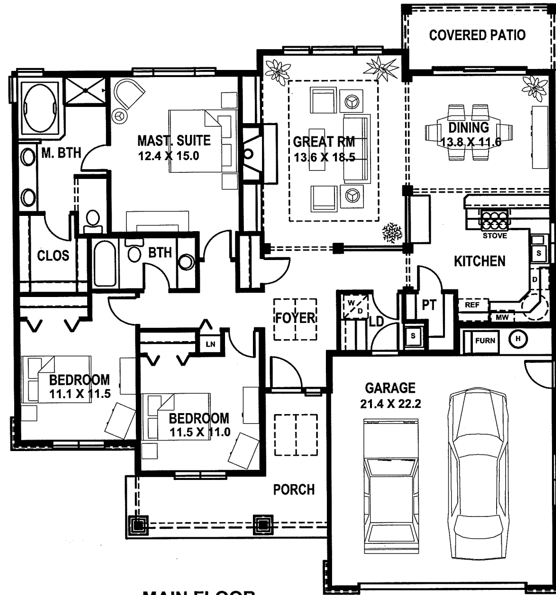
MAIN FLOOR 1696 sf
